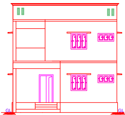
FRONT ELEVATION
