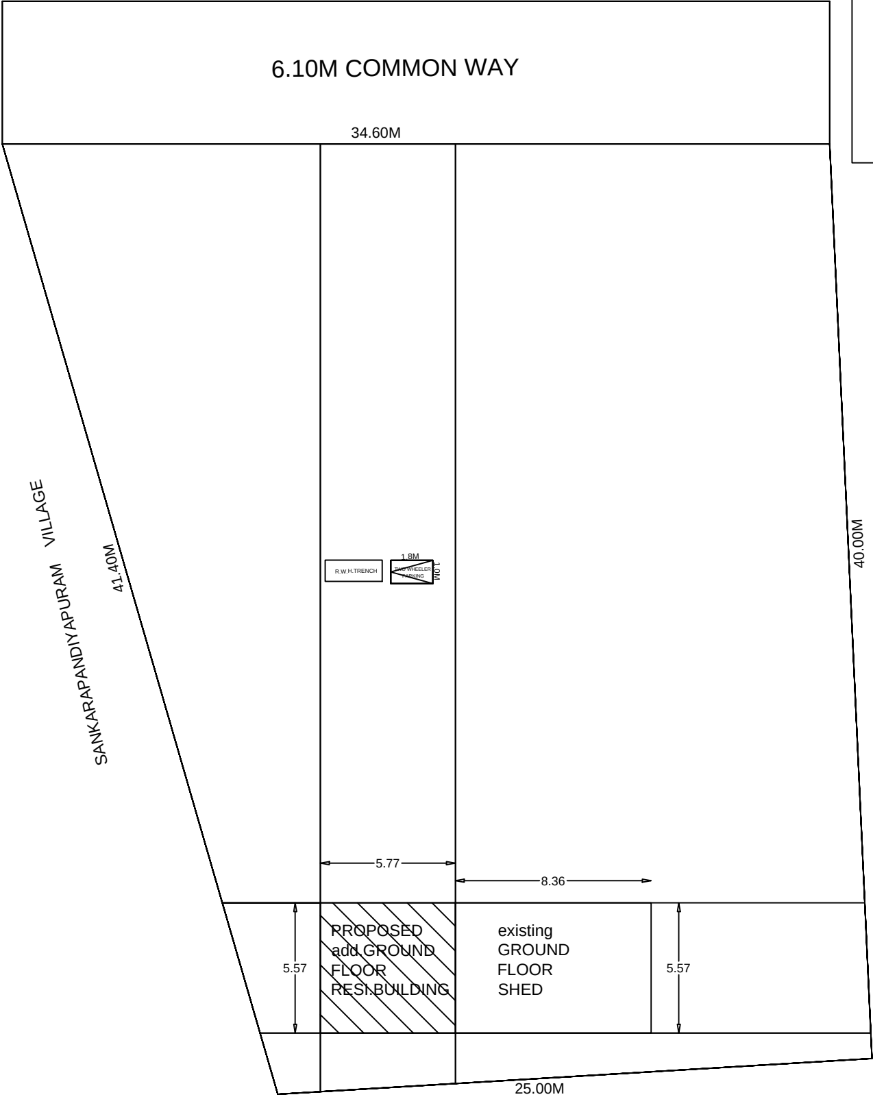
SITE PLAN
