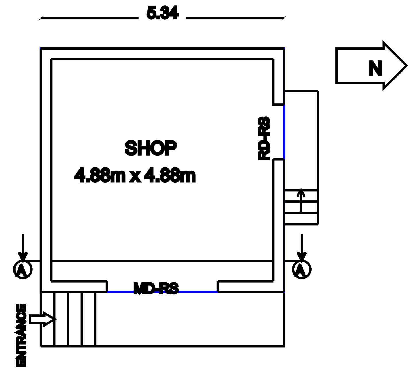
FLOOR PLAN
