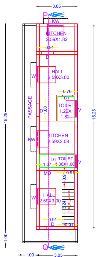
PROPOSED SECOND FLOOR PLAN
