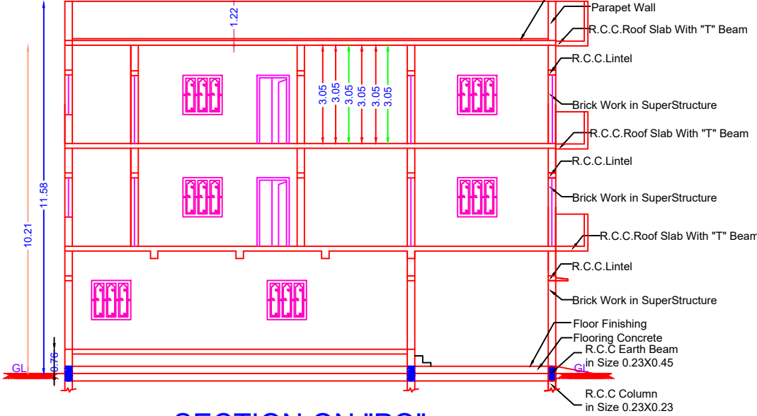
SECTION ON "PQ" (SCALE 1:100)
