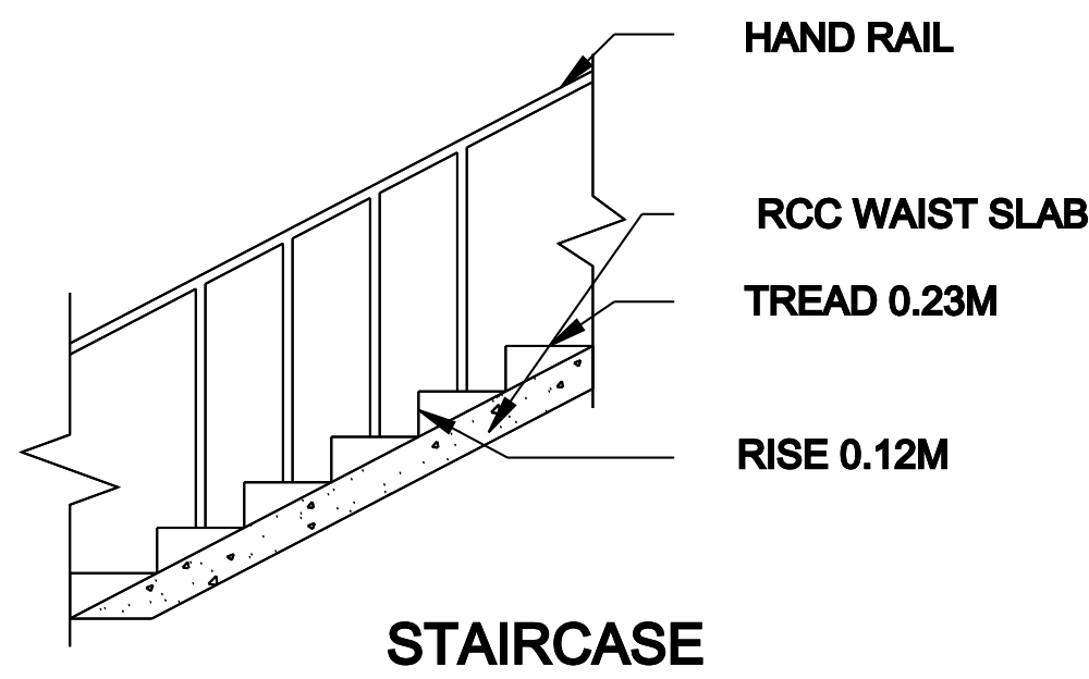
STAIRCASE
