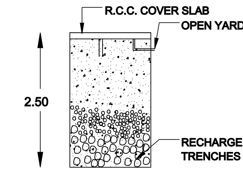
SECTION C-C'
