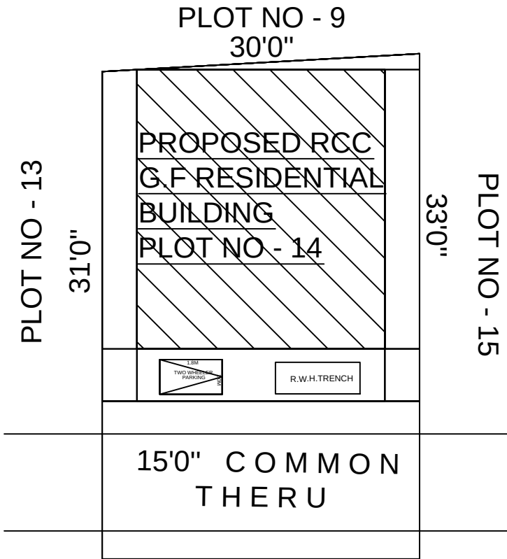
SITE PLAN
