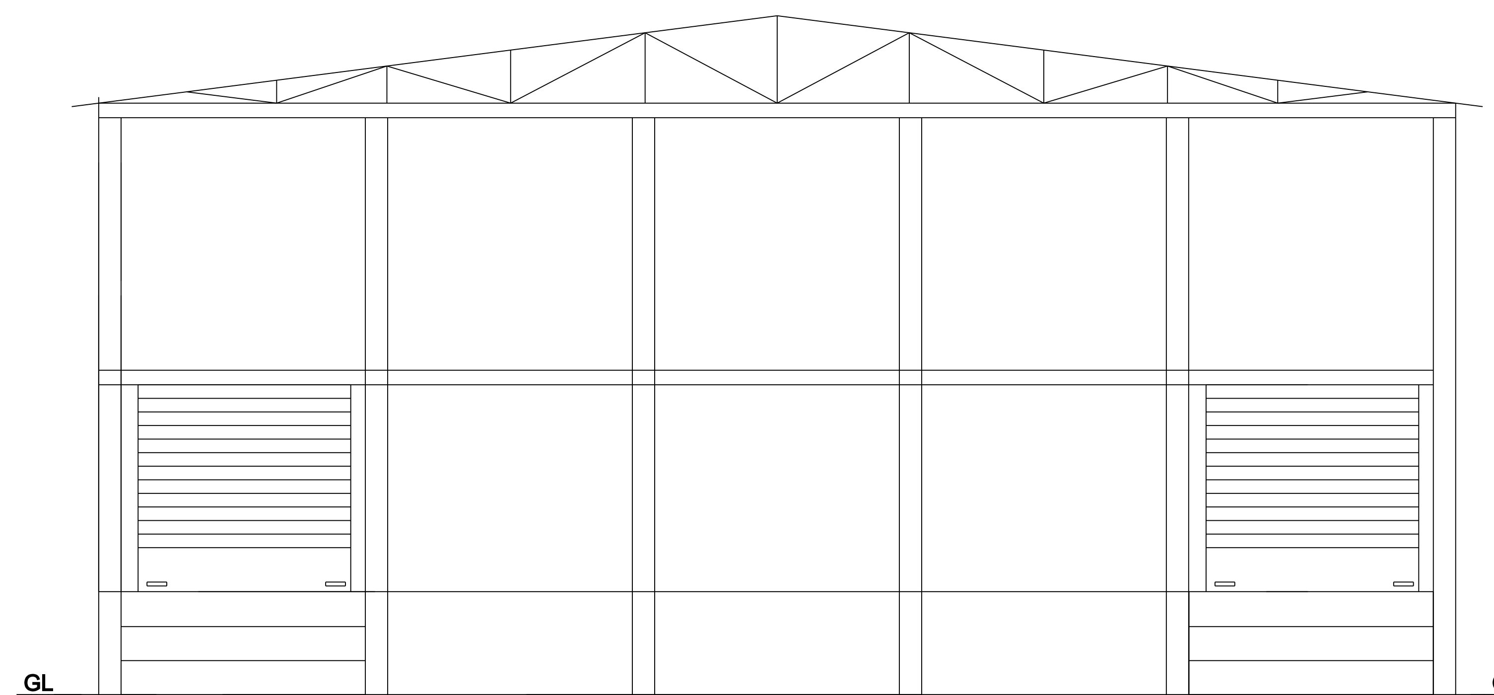
FRONT ELEVATION
