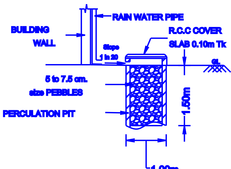
RAIN WATER HARVESTING TRENCH PIT DETAILS
