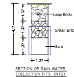
SECTION OF RAIN WATER COLLECTION PITS (R.W.C.)
