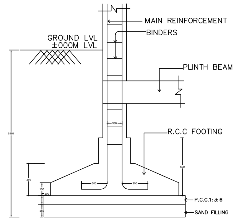
TYPICAL SECTION OF R.C.C COLUMN FOUNDATION
