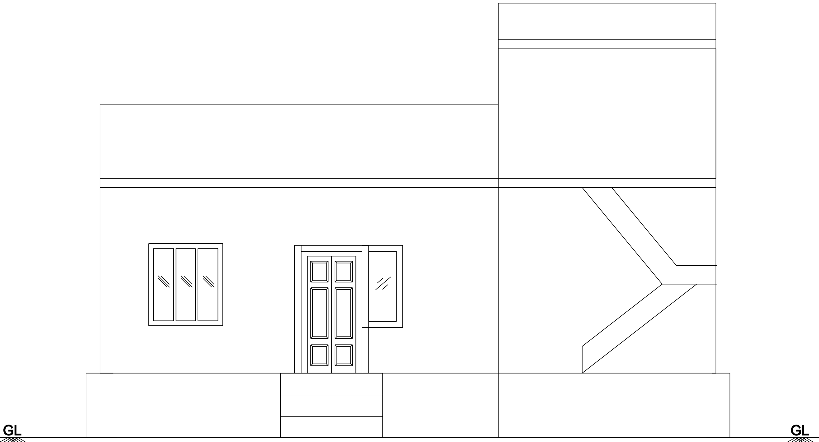
FRONT ELEVATION
