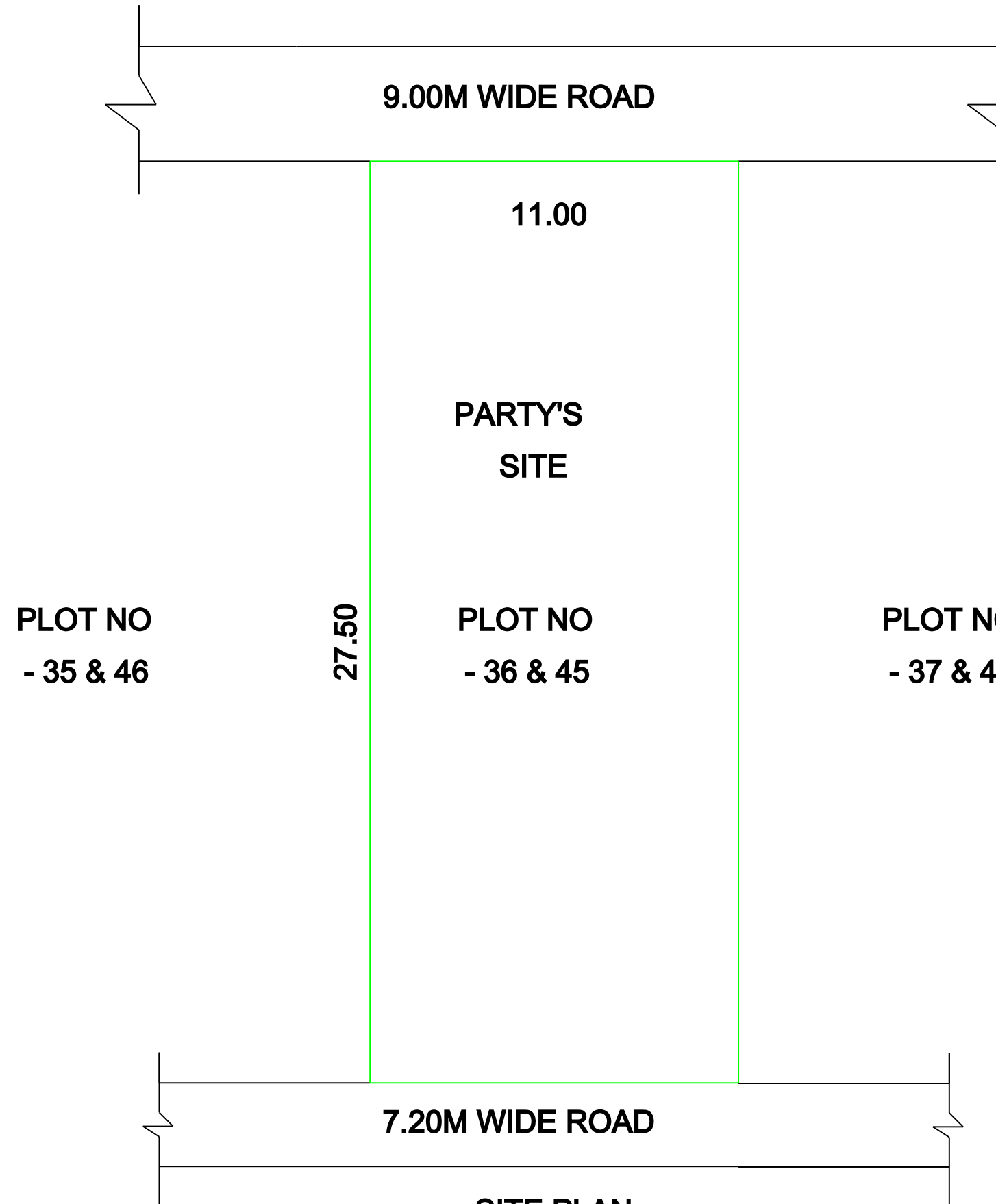
SITE PLAN
