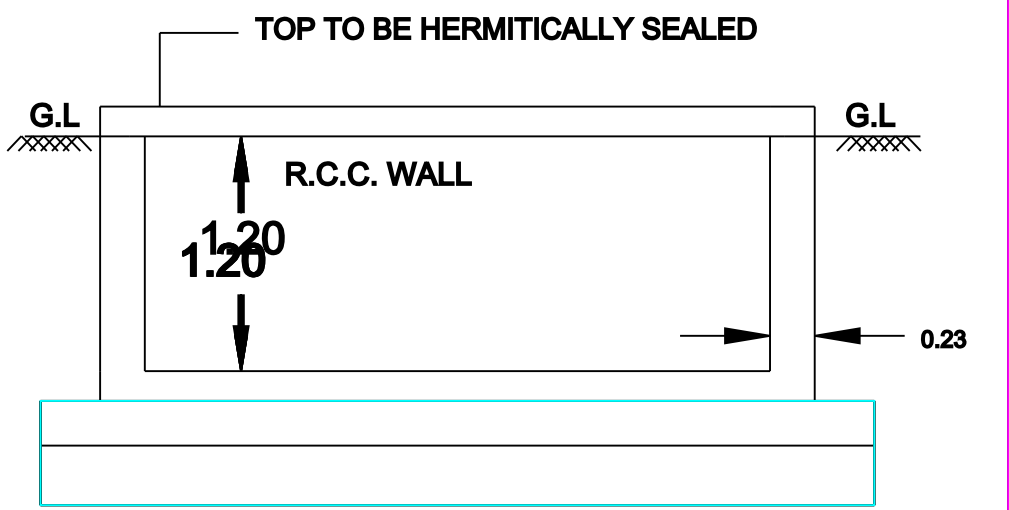
RWH SECTION
