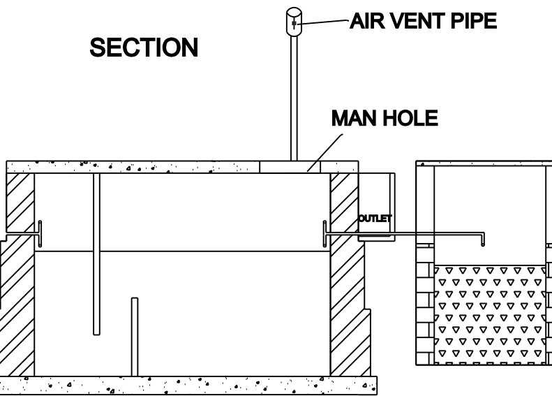
SECTION
