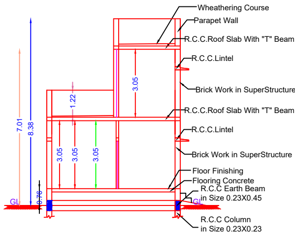
SECTION ON "PQ" (SCALE 1:100)
