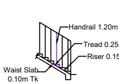
DETAILS OF STAIR CASE (SCALE 1:100)
