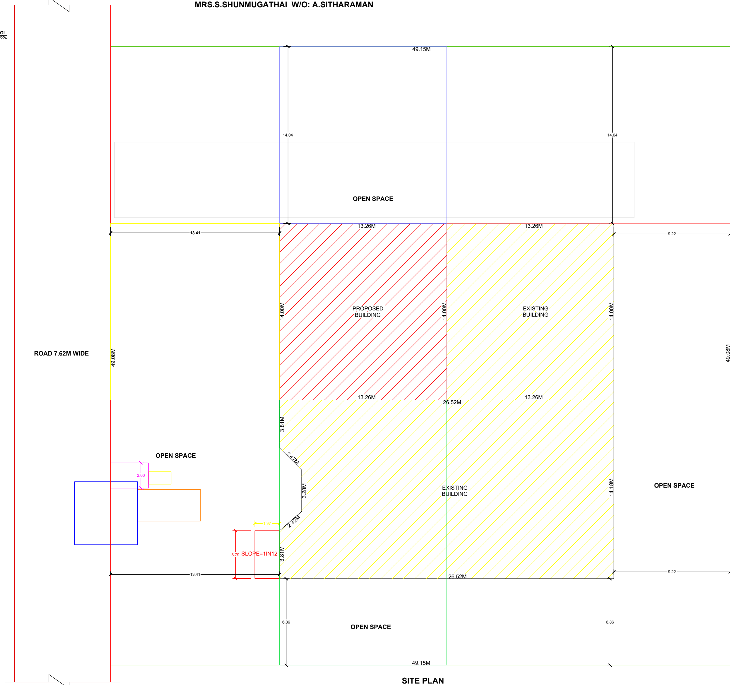
SITE PLAN
