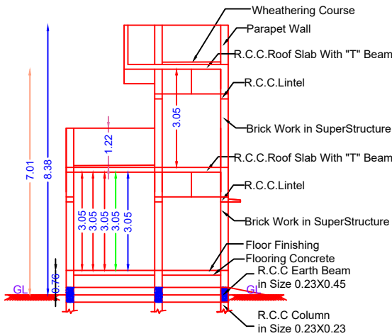
SECTION ON "PQ" (SCALE 1:100)
