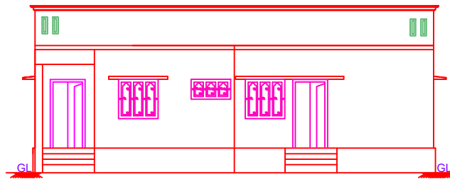
FRONT ELEVATION
