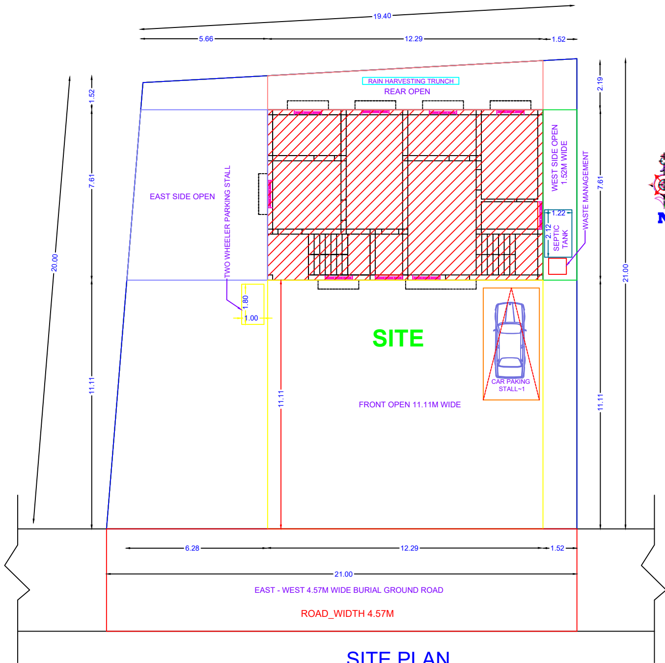
SITE PLAN
