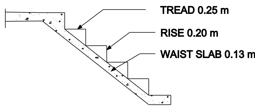
STAIR DETAILS
