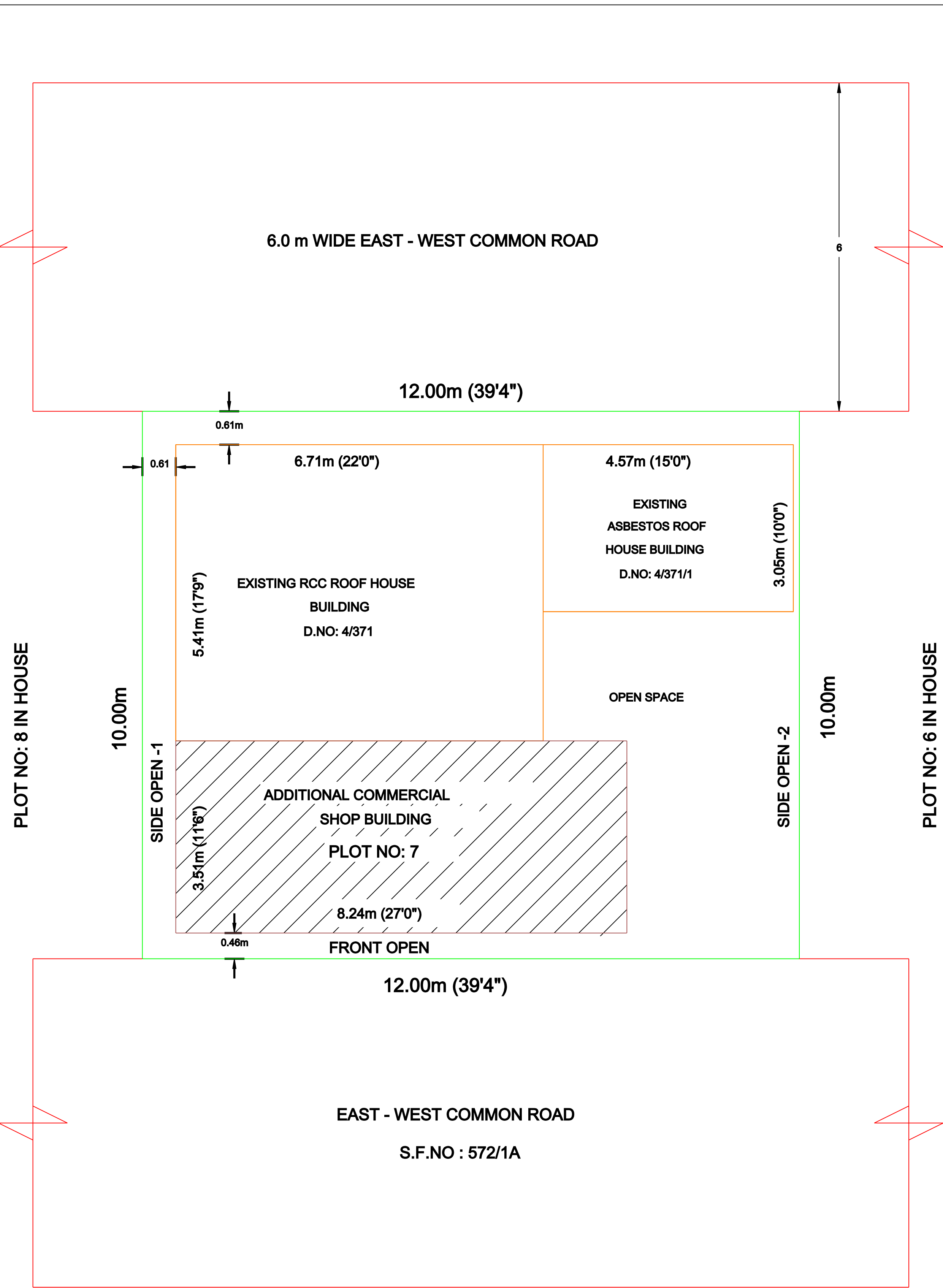
SITE PLAN
