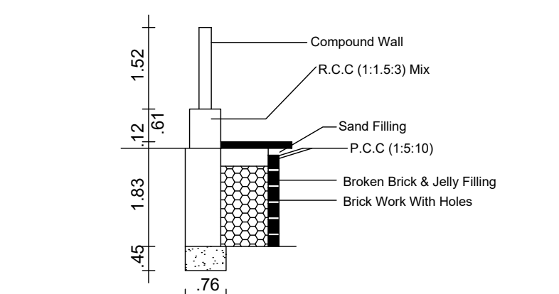
RAIN WATER HARVEST DETAILS
