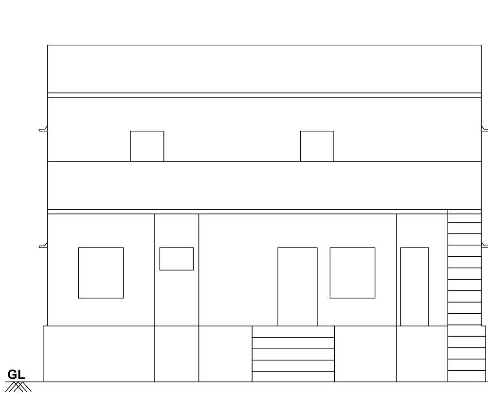
EASTERN SIDE ELEVATION
