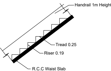
STAIR DETAILS
