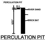
PERCULATION PIT
