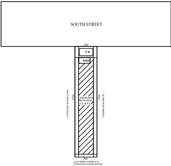
SITE PLAN
