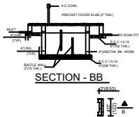
TANK
