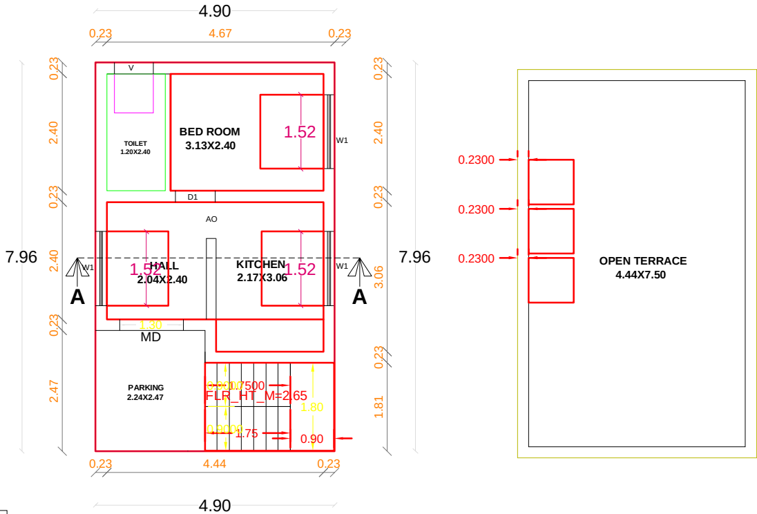
TERRACE FLOOR PLAN PROPOSED
