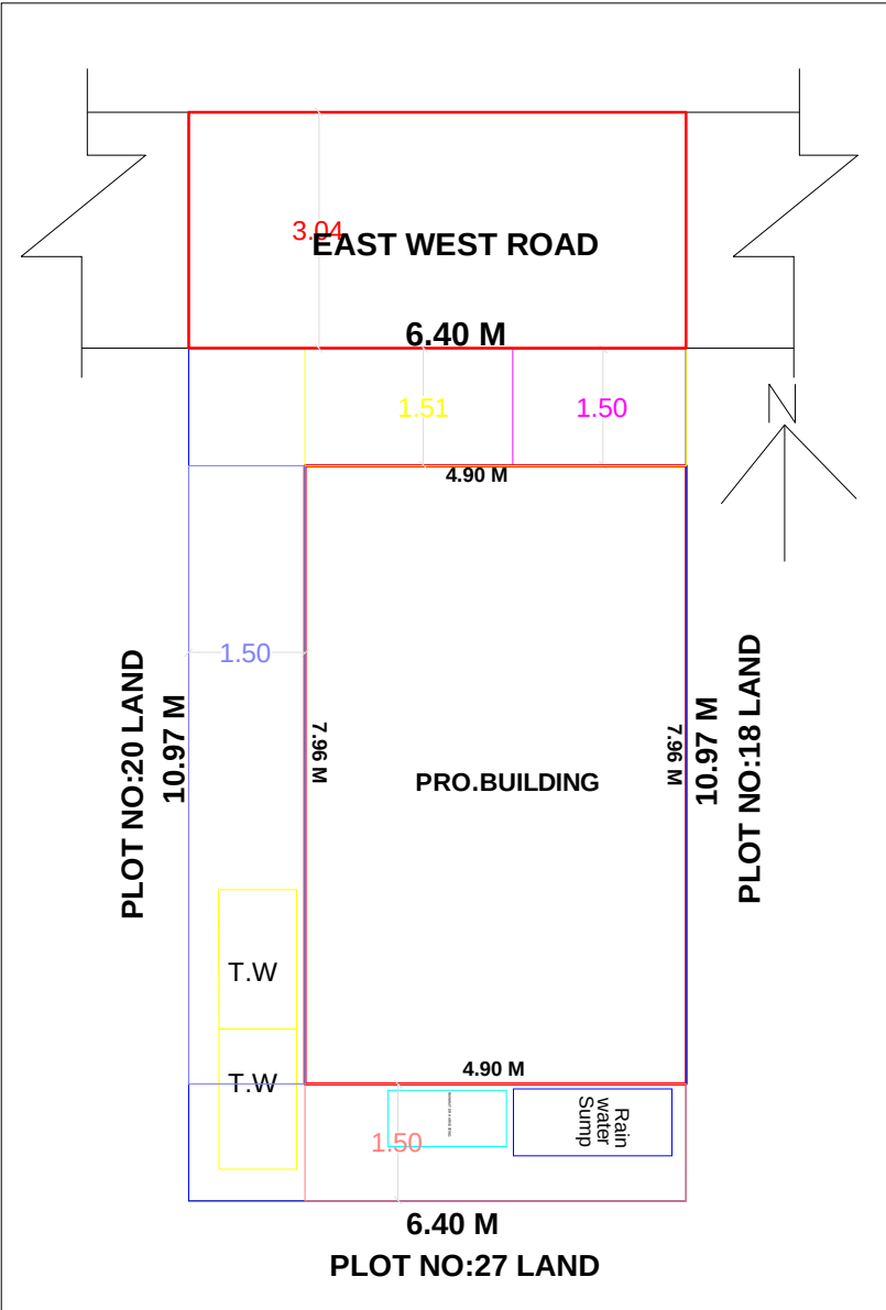
SITE FLOOR PLAN PROPOSED
