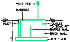
SECTION OF SEPT.TANK
