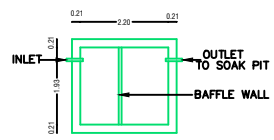
PLAN SEPTIC. TANK
