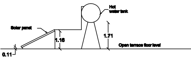
SIDE ELEVATION
