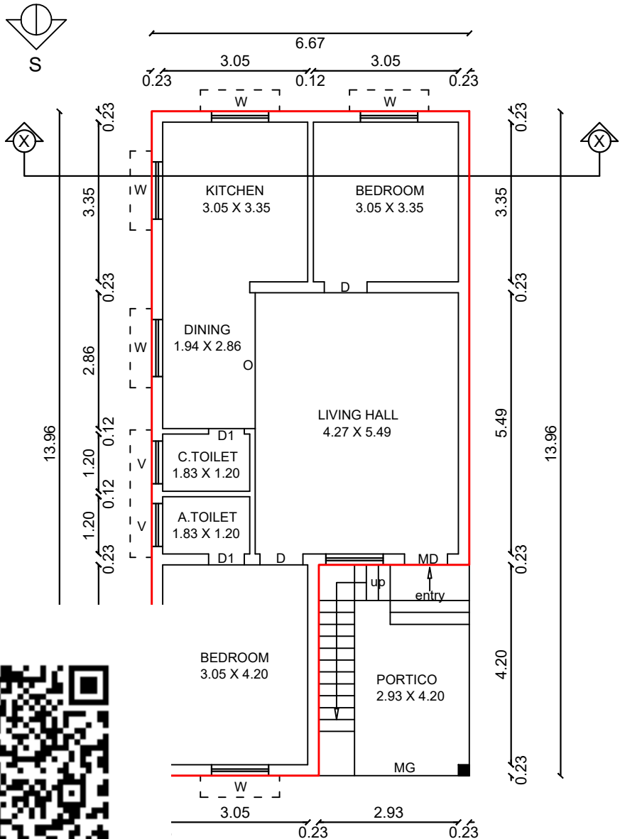
ROPOSED GROUND FLOOR PLAN
