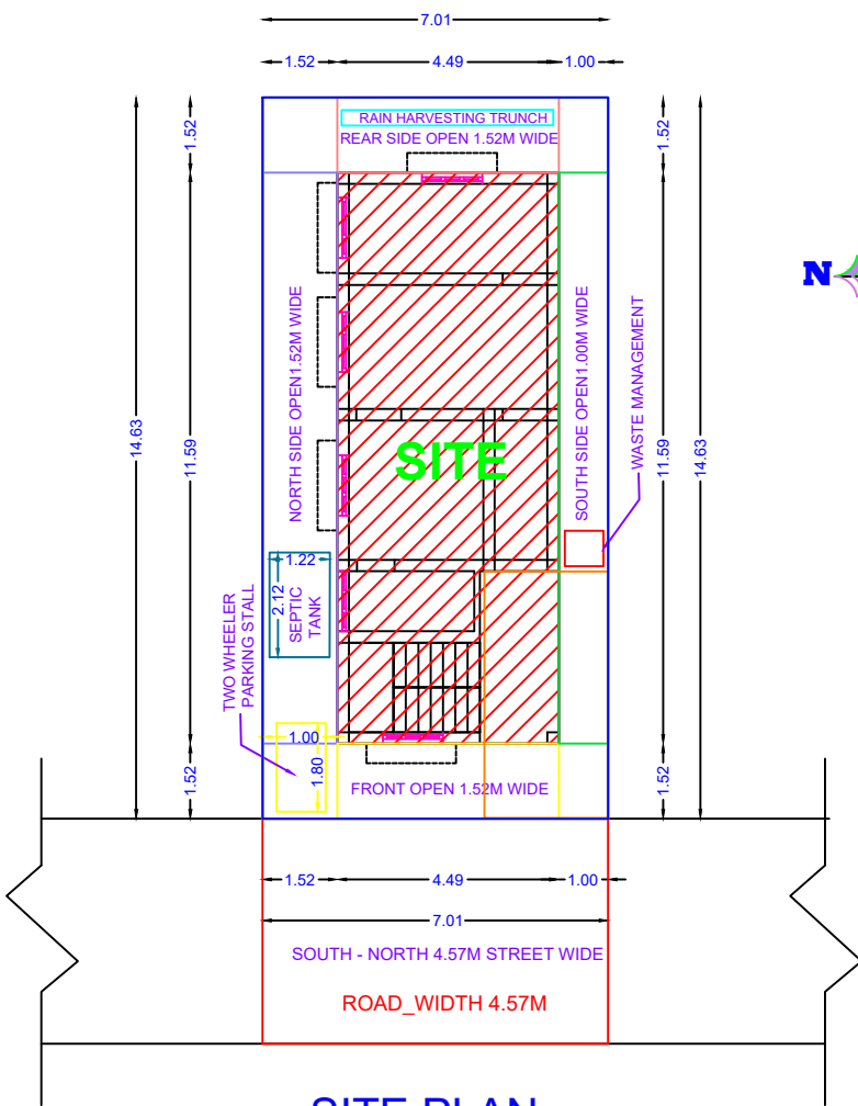
SITE PLAN
