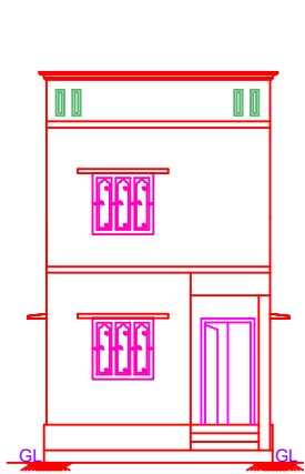
FRONT ELEVATION
