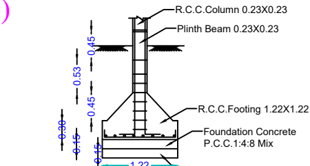
DETAILS OF COLUMN FOOTING (SCALE 1:50)
