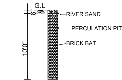
PERCOLATION PIT
