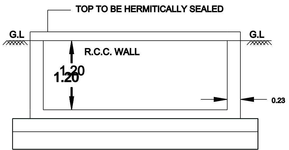
RWH SECTION
