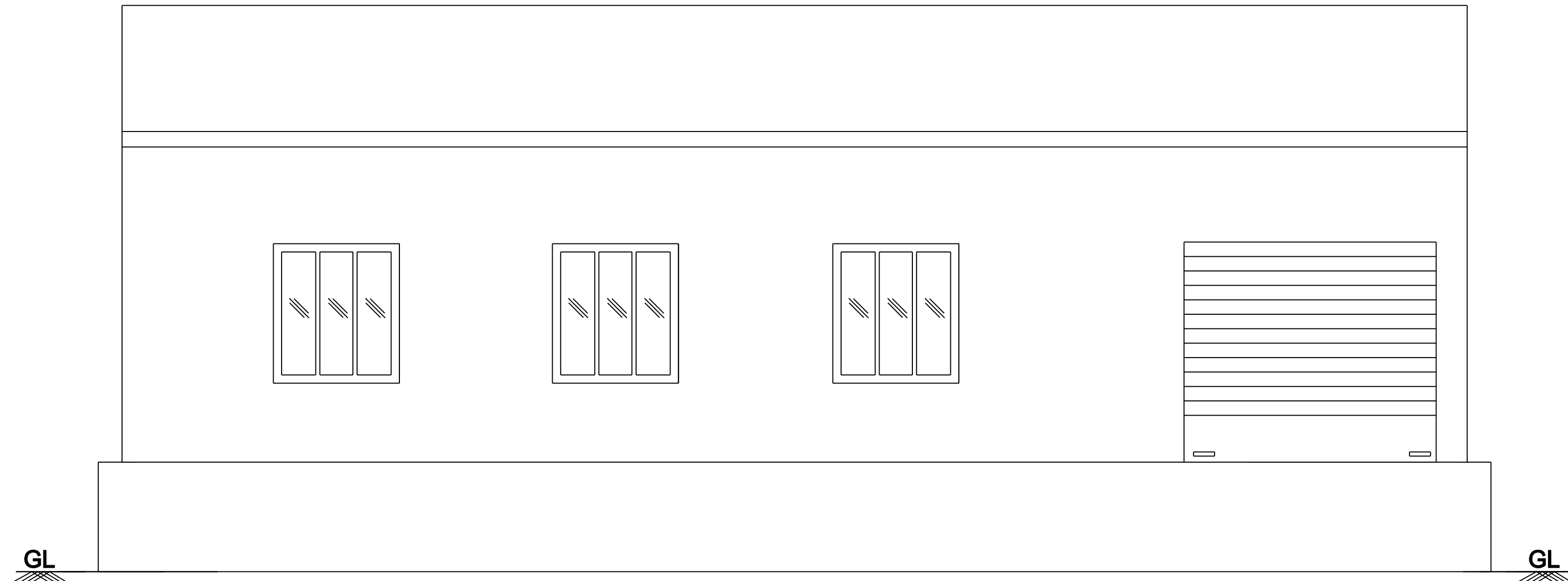
FRONT ELEVATION
