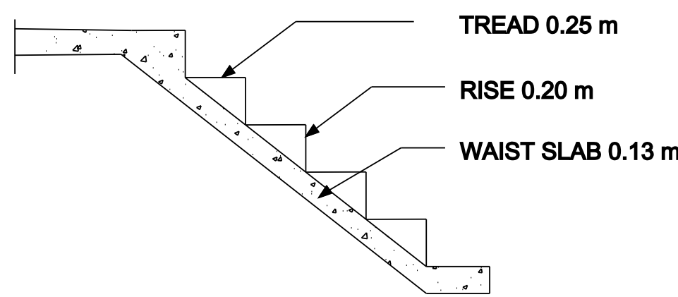
STAIR DETAILS
