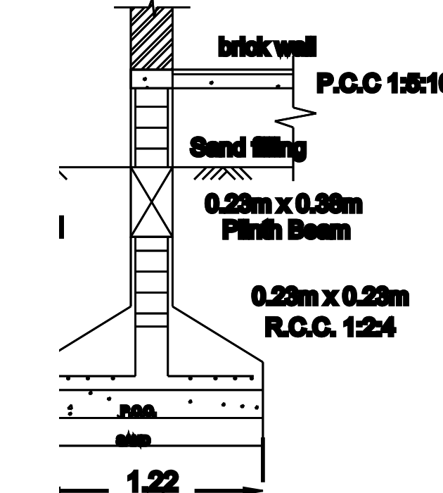
FOUNDATION DETAILS
