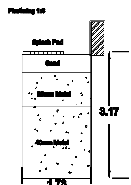
RAIN WATER PERCOLATION PIT
