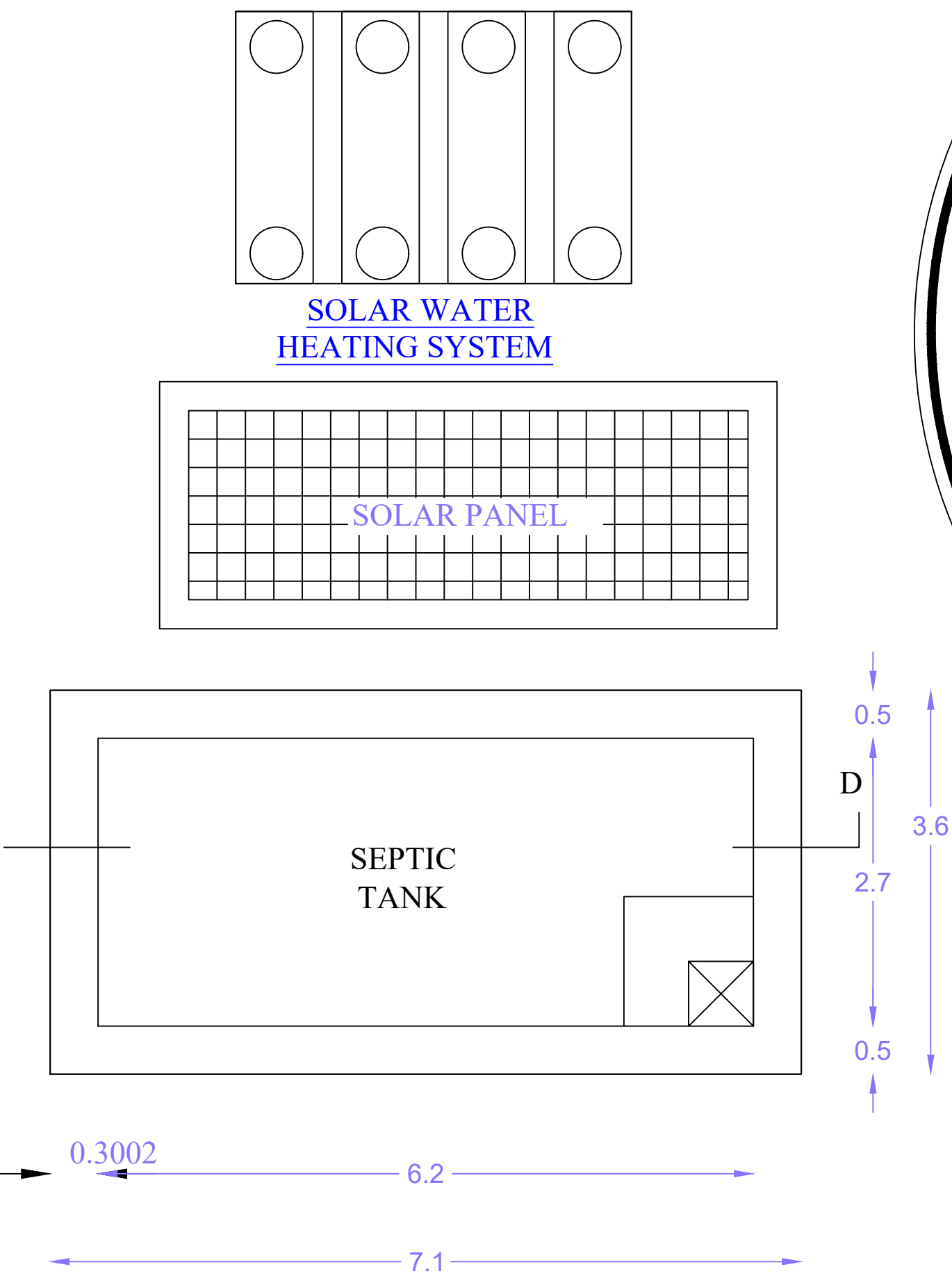
PLAN OF SEPTIC TANK SCALE 1"=2'-0"
