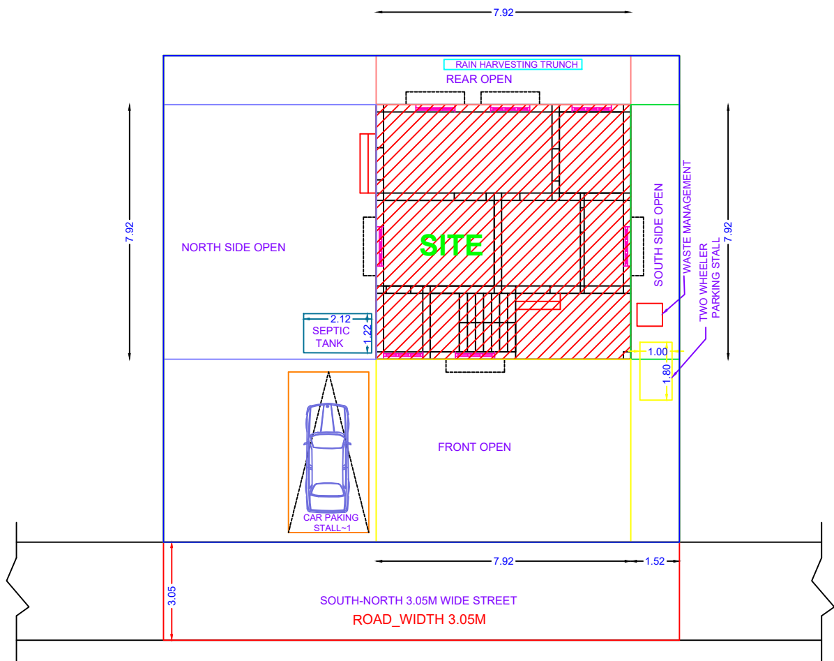
SITE PLAN
