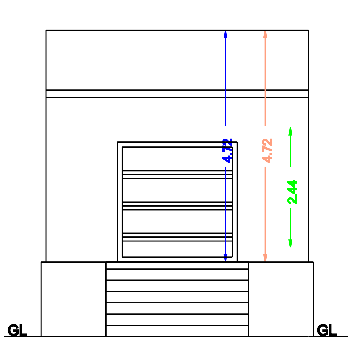
WESTERN SIDE FRONT ELEVATION
