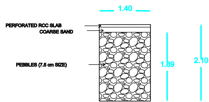
RAIN WATER HARVESTING
