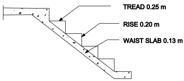
STAIR DETAILS
