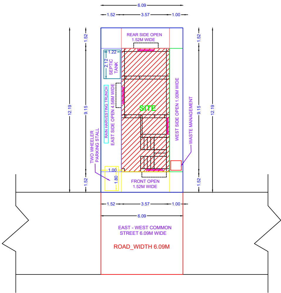
SITE PLAN
