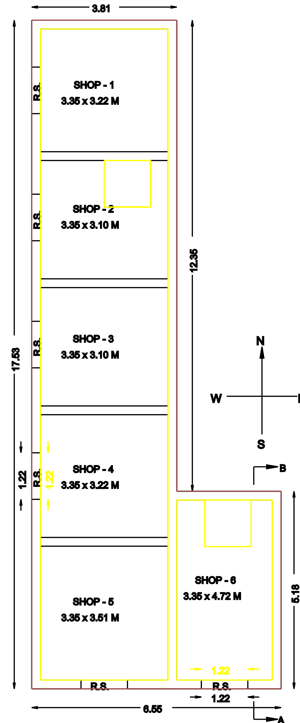
PROPOSED BUILDING PLAN
