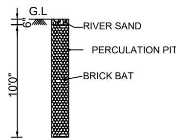
PERCULATION PIT
