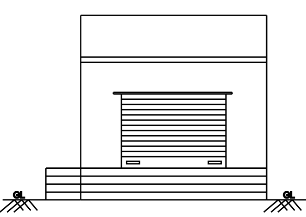
FRONT ELEVATION S.P.M. TRADERS
