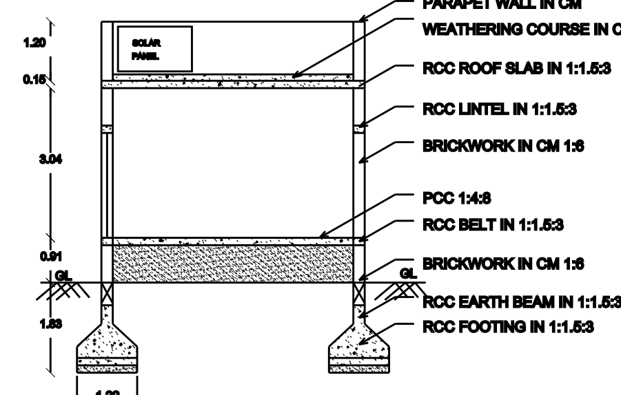
SECTION ON 'AA' S.P.M. CRACKERS
