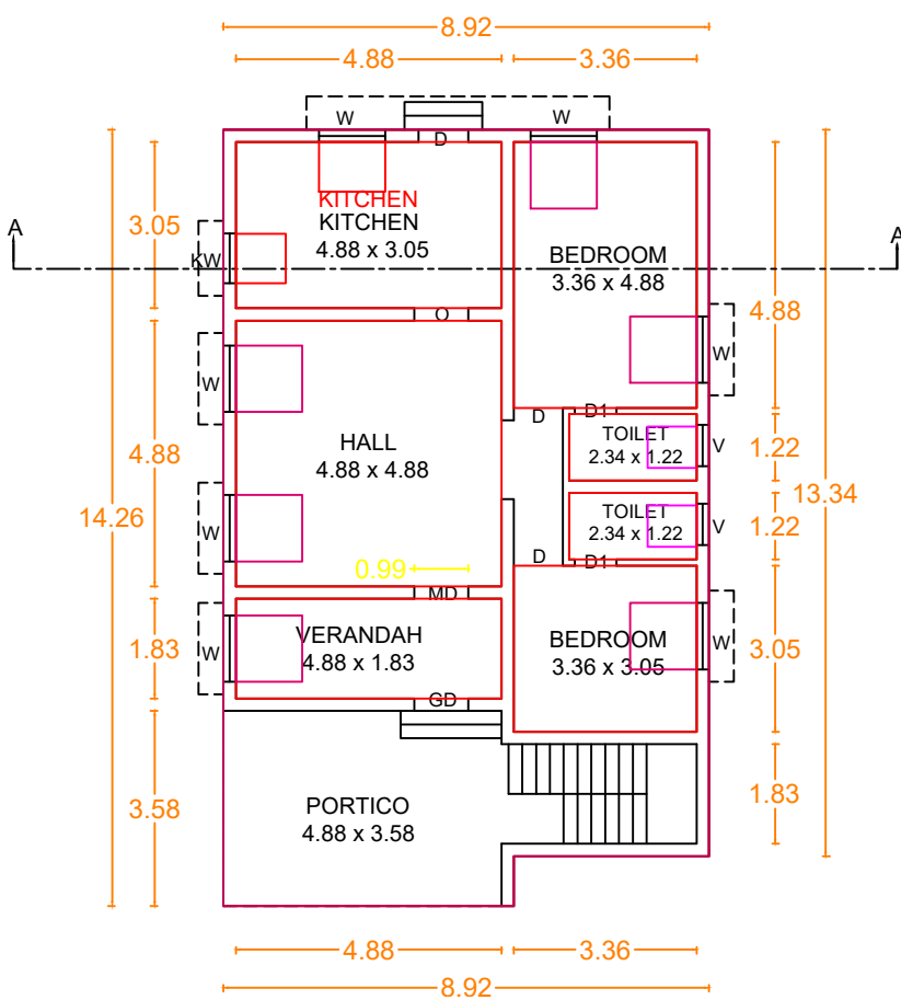
FLOOR PLAN
