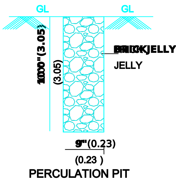
PERCOLATION PIT
