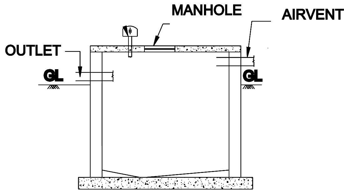
SECTION B-B'
