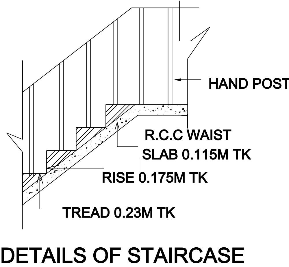
DETAILS OF STAIRCASE
