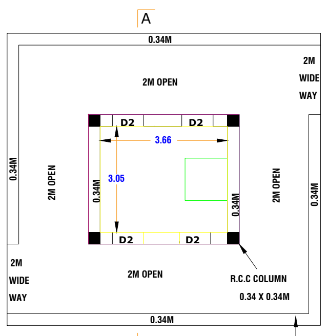
PLAN-3
