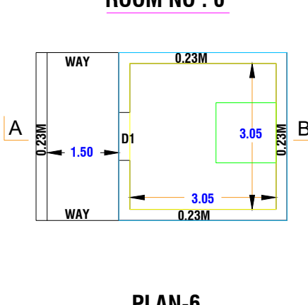
PLAN-6
