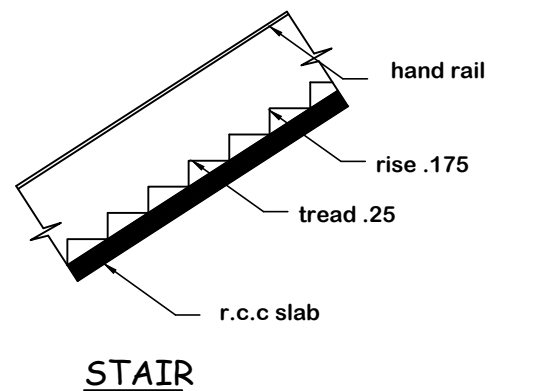
STAIR
