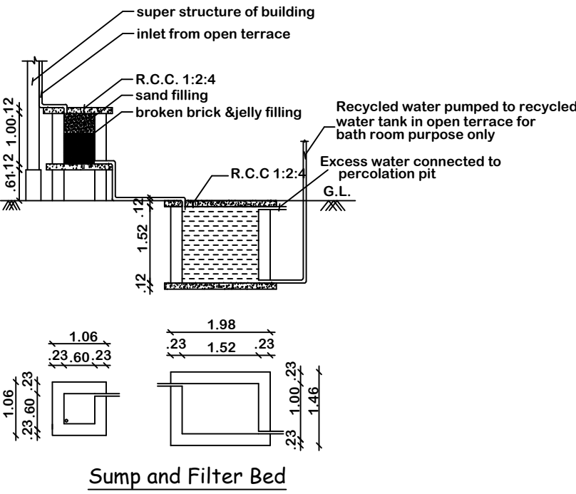
Sump and Filter Bed
