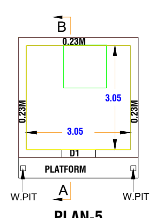
PLAN-5
