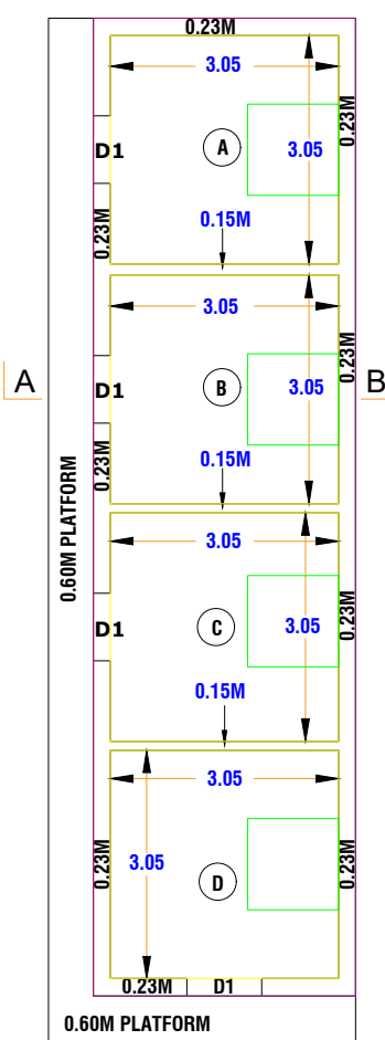
PLAN-4
