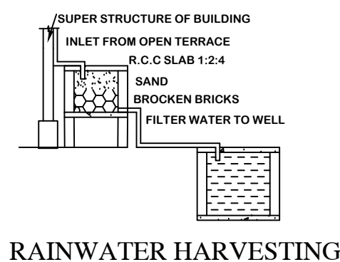
RAINWATER HARVESTING
