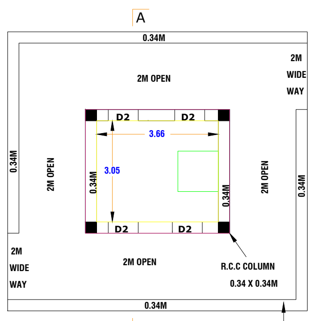
PLAN-1
