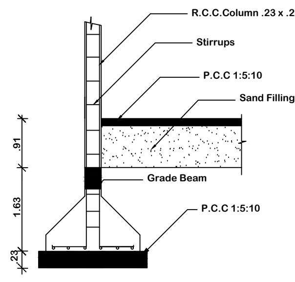
COLUMN DETAIL
