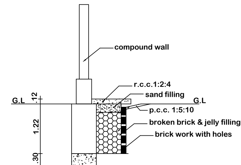
PLINTH BOUNDARY PERCOLATION PIT
