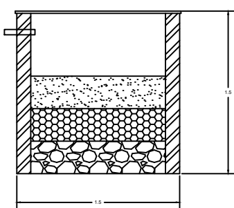
RAIN WATER TANK
