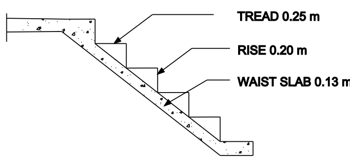
STAIR DETAILS
