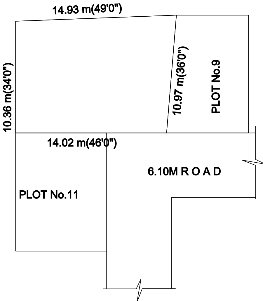
LOCATION PLAN SCALE :- 1:400
