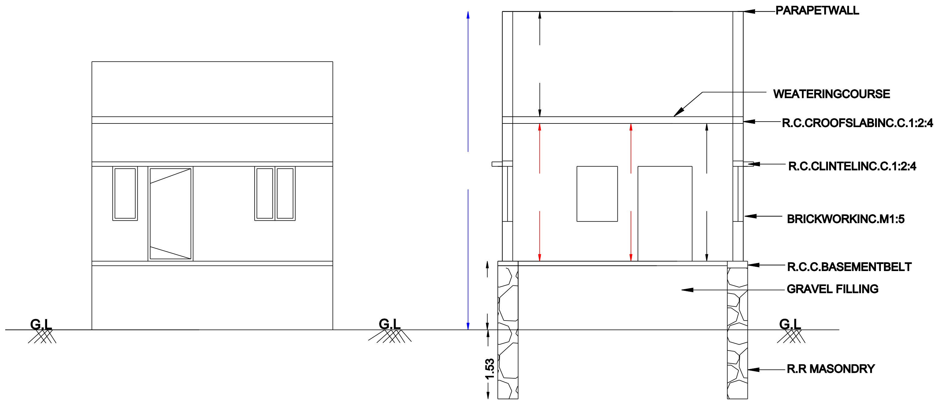
FRONT ELEVATION
