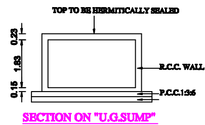
SECTION ON "U.G.SUMP"
