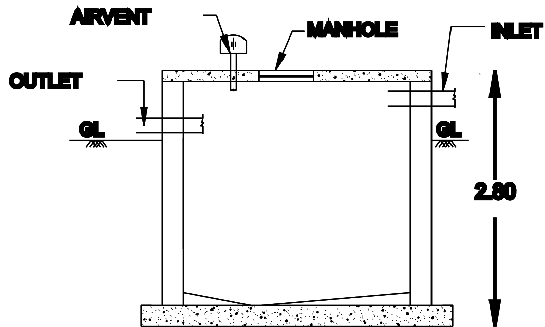
SECTION B-B'
