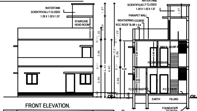
SECTION "A-B"
