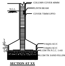
SECTION AT XX
