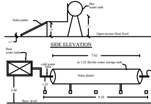
SOLAR WATER HEATER PLANT
