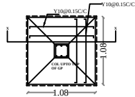
COLUMN (C1)
