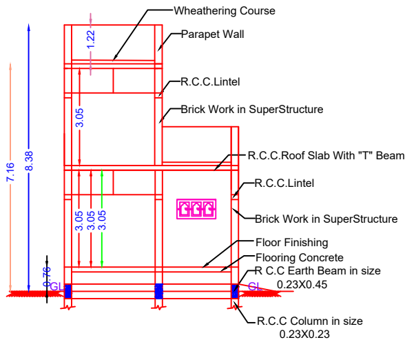
SECTION ON "PQ" SCALE 1:100
